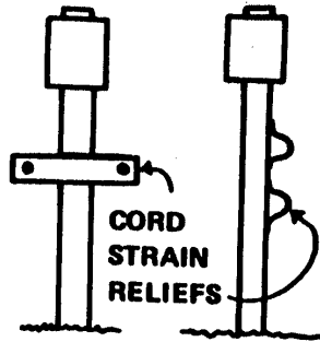
TYPICAL RV LOAD CENTERS WITH DIFFERENT CORD STRAIN RELIEFS
