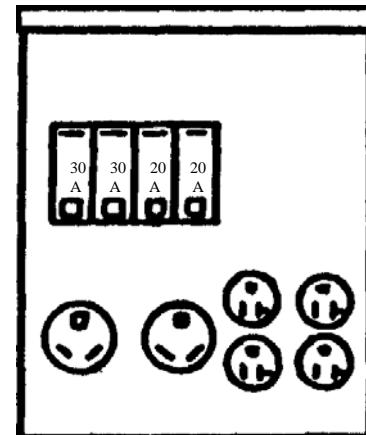
Type C Dual campsite load center with 20 and 30 ampere receptacles. Each of the two RV units using the panel are limited to a maximum of 24 amperes. This type used only in older campgrounds.
