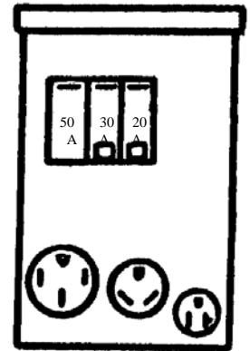
Type B Single campsite load center With 20, 30 and 50 ampere receptacles. RV is limited to a maximum of 40 amperes.
