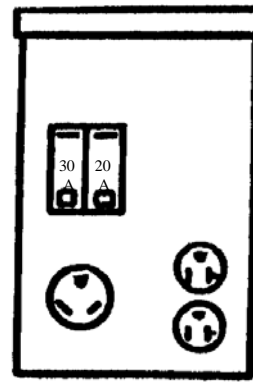
Type A Single campsite load center with 20 and 30 ampere receptacles. RV is limited to a maximum of 24 amperes.
